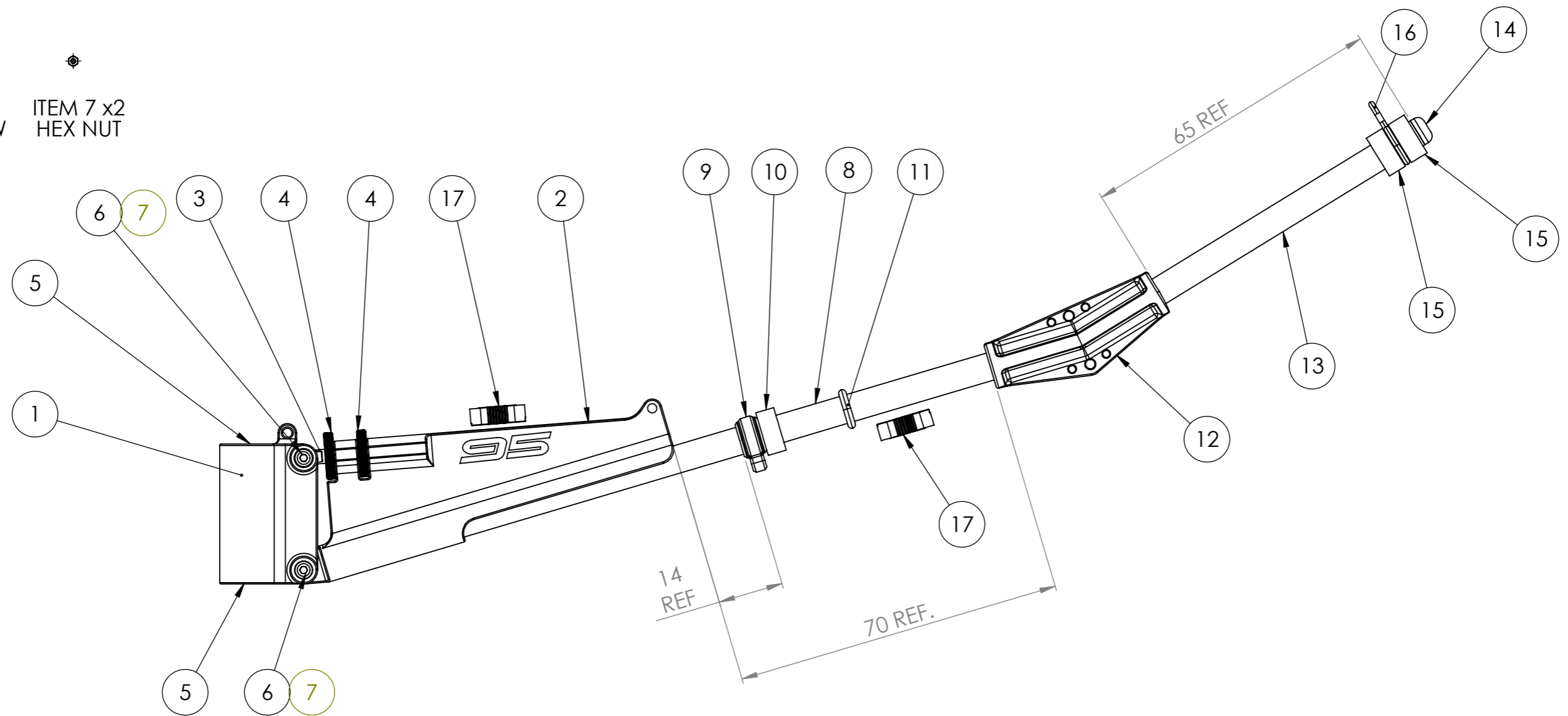
DF95 MAIN BOOM KIT ASSEMBLY 'C'
