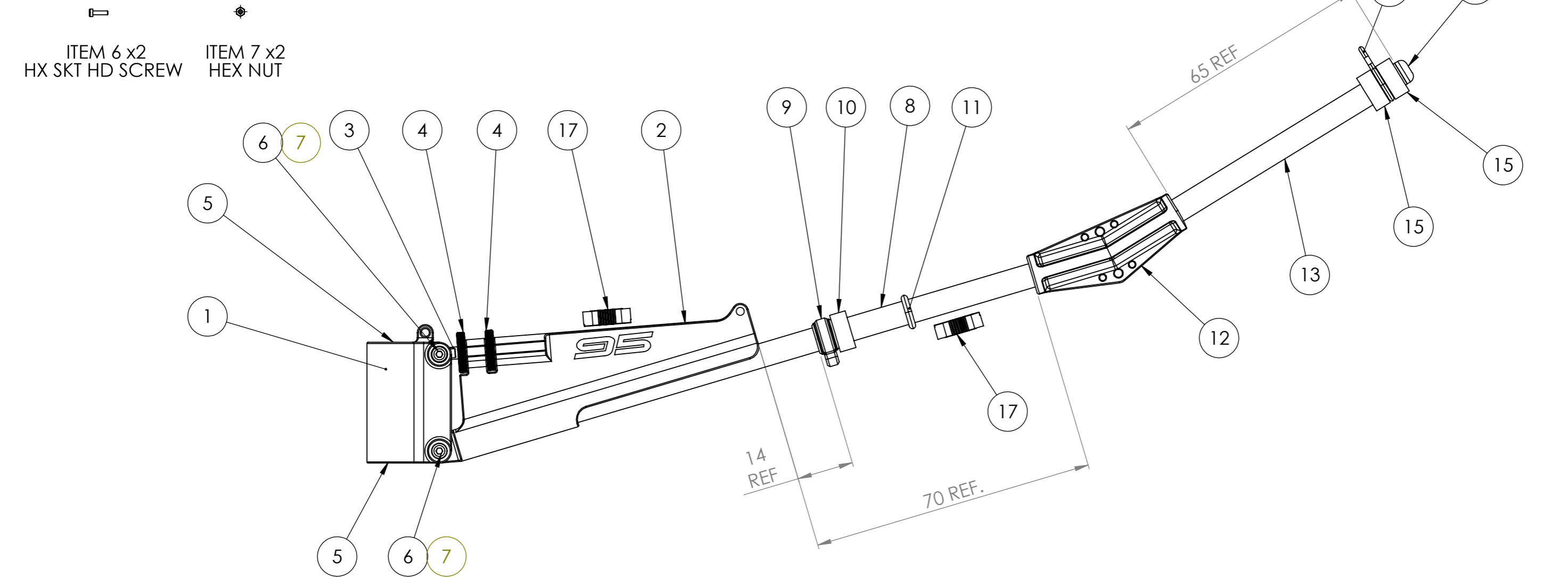
DF95 MAIN BOOM KIT ASSEMBLY 'C'
