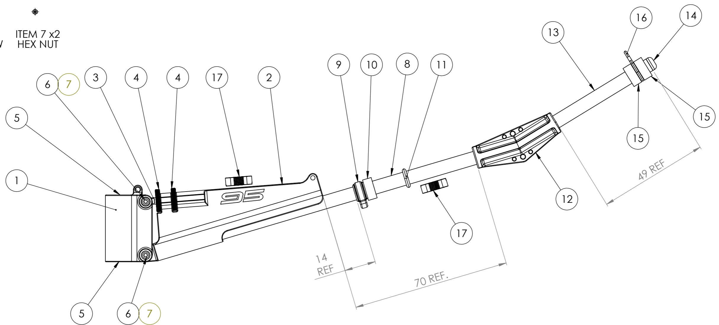
DF95 MAIN BOOM KIT ASSEMBLY 'D'
